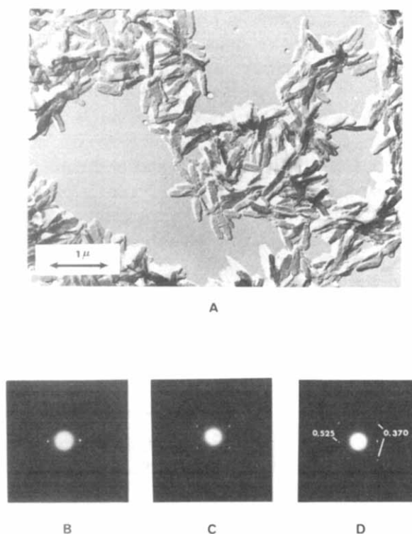
Fig. 1. (A) Transmission electron micrograph of A amylose crystals shadowed with tungsten-tantalum. (B-D) Typical electron diffraction patterns obtained from individual platelet crystals as in (A) but unshadowed and examined in the frozen hydrated state.
