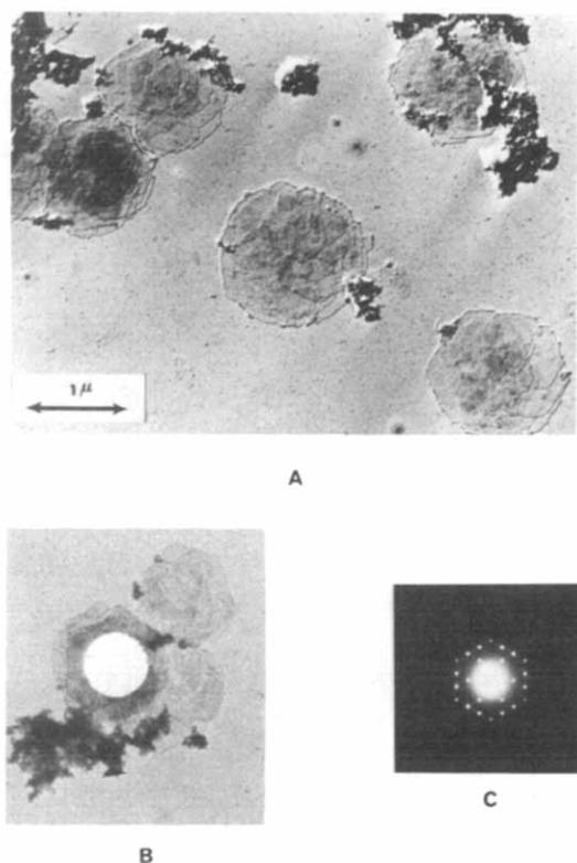
Fig. 4. (A) Transmission electron micrograph of V amylose crystals shadowed with tungsten-tantalum. (B) Transmission electron micrograph of a cluster of unshadowed V amylose crystals in a frozen hydrated state. (C) Electron diffraction pattern (correctly oriented) recorded from the circled area of Fig. 4(B).
